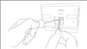
Fig. 4 Connect the pair of cables from the BUS BridgeNet on the boiler circuit board to the BUS BridgeNet connector on REMOCON NET MINI (observing the polarities B to B and T to T)* *to facilitate cable connection, the plastic tab can be removed as shown in the diagram.
