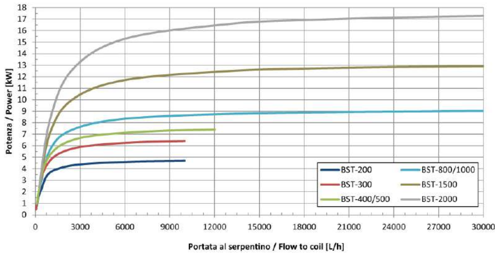
Potenza scambiata, scamb. integrazione T_{in,coil} = 50\text{ }^{\circ}\text{C} ; T_{serb,in} = 10\text{ }^{\circ}\text{C} , T_{serb,out} = 45\text{ }^{\circ}\text{C}
