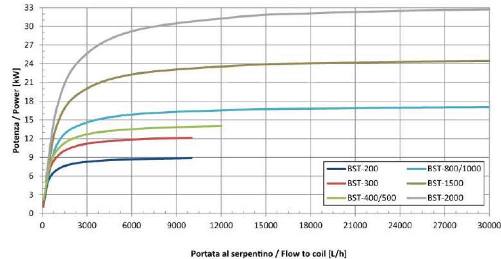
Potenza scambiata, scamb. integrazione T_{in,coil} = 60\text{ }^{\circ}\text{C} ; T_{serb,in} = 10\text{ }^{\circ}\text{C} , T_{serb,out} = 45\text{ }^{\circ}\text{C}
