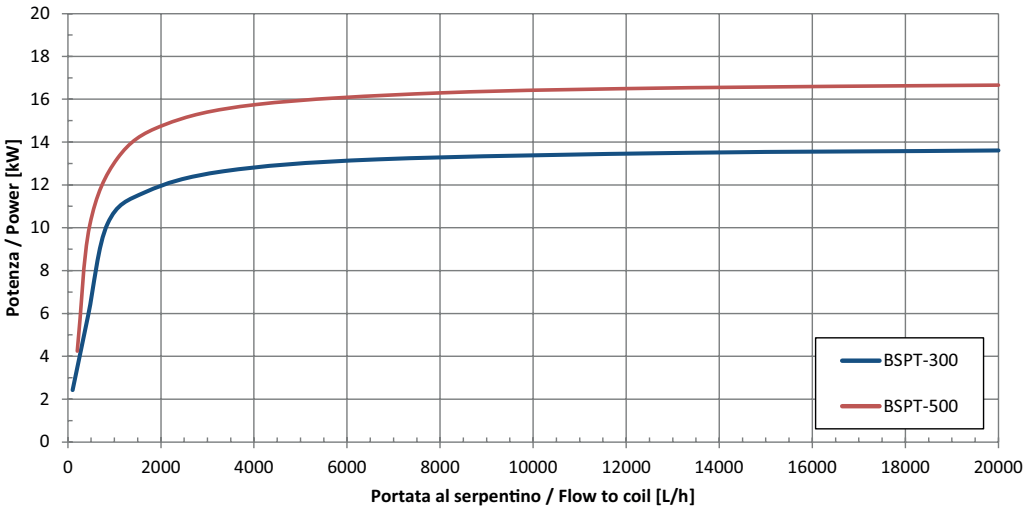
Potenza scambiata, scamb.integr. T_{in,coil} = 80\text{ }^{\circ}\text{C} ; T_{serb,in} = 10\text{ }^{\circ}\text{C} , T_{serb,out} = 45\text{ }^{\circ}\text{C}
