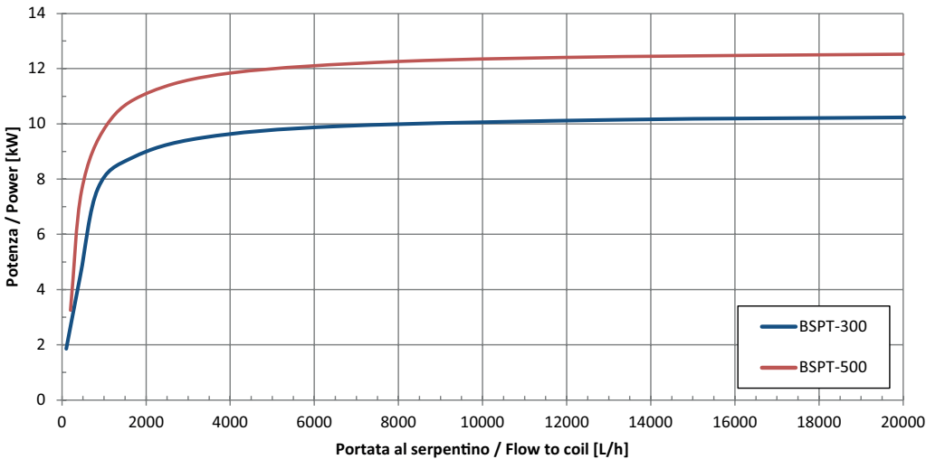
Potenza scambiata, scamb.integr. T_{in,coil} = 70\text{ }^{\circ}\text{C} ; T_{serb,in} = 10\text{ }^{\circ}\text{C} , T_{serb,out} = 45\text{ }^{\circ}\text{C}
