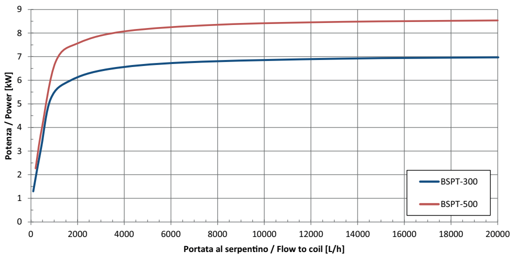
Potenza scambiata, scamb.integr. T_{in,coil} = 60\text{ }^{\circ}\text{C} ; T_{serb,in} = 10\text{ }^{\circ}\text{C} , T_{serb,out} = 45\text{ }^{\circ}\text{C}
