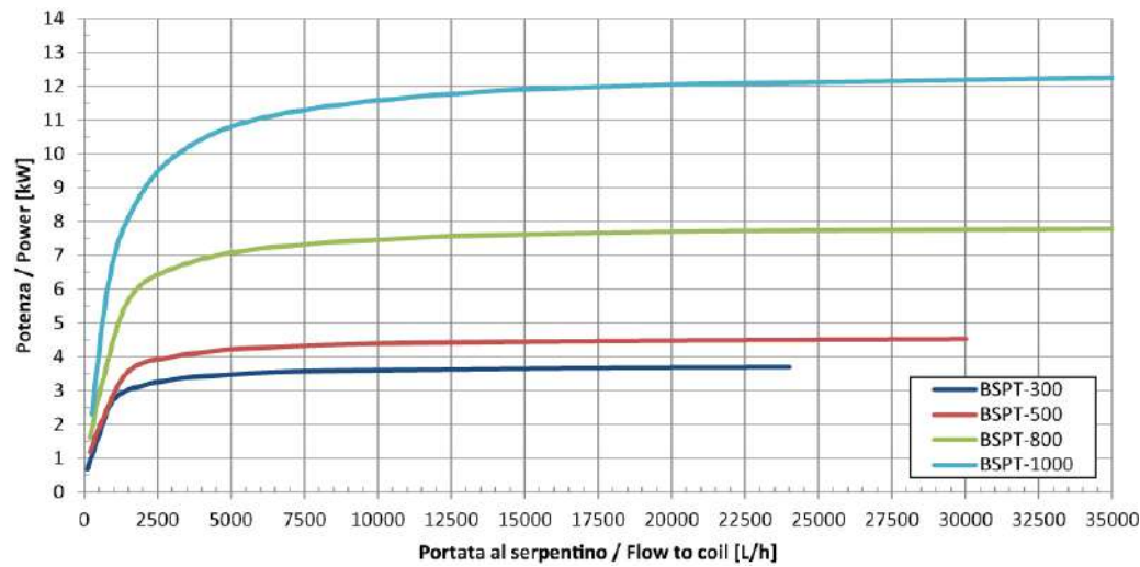
Potenza scambiata, scamb. integrazione T_{in,coil} = 50\text{ }^{\circ}\text{C} ; T_{serb,in} = 10\text{ }^{\circ}\text{C} , T_{serb,out} = 45\text{ }^{\circ}\text{C}
